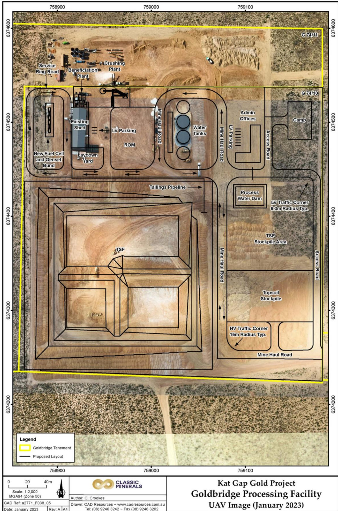
Figure 2: Overlay of design on aerial photo of Kat Gap Processing Facility.
