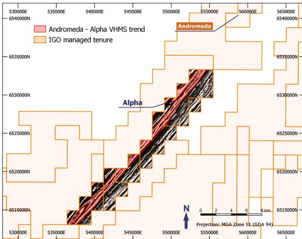
Figure 5: Interpreted Andromeda / Alpha host horizon
